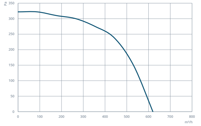
CUB 160
