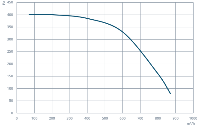
SAF 15
