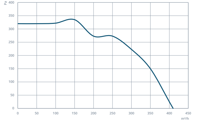
CUB 125
