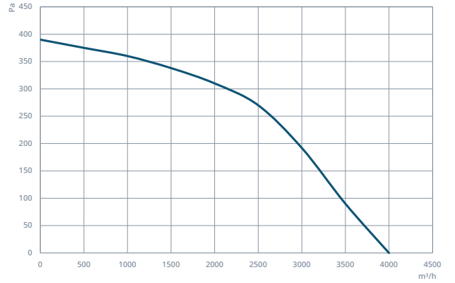
IGK 40
