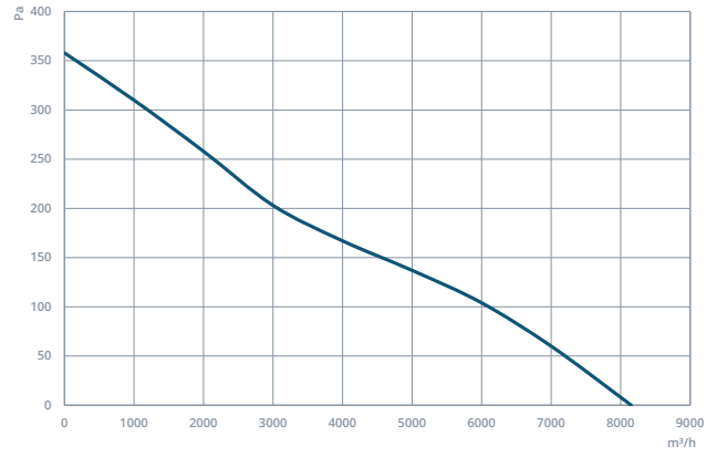
HAXI 560-5-25
