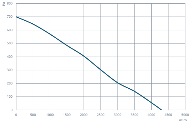
SHU 43
