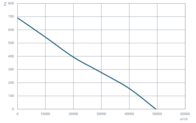
BAXI 1000-5-40
